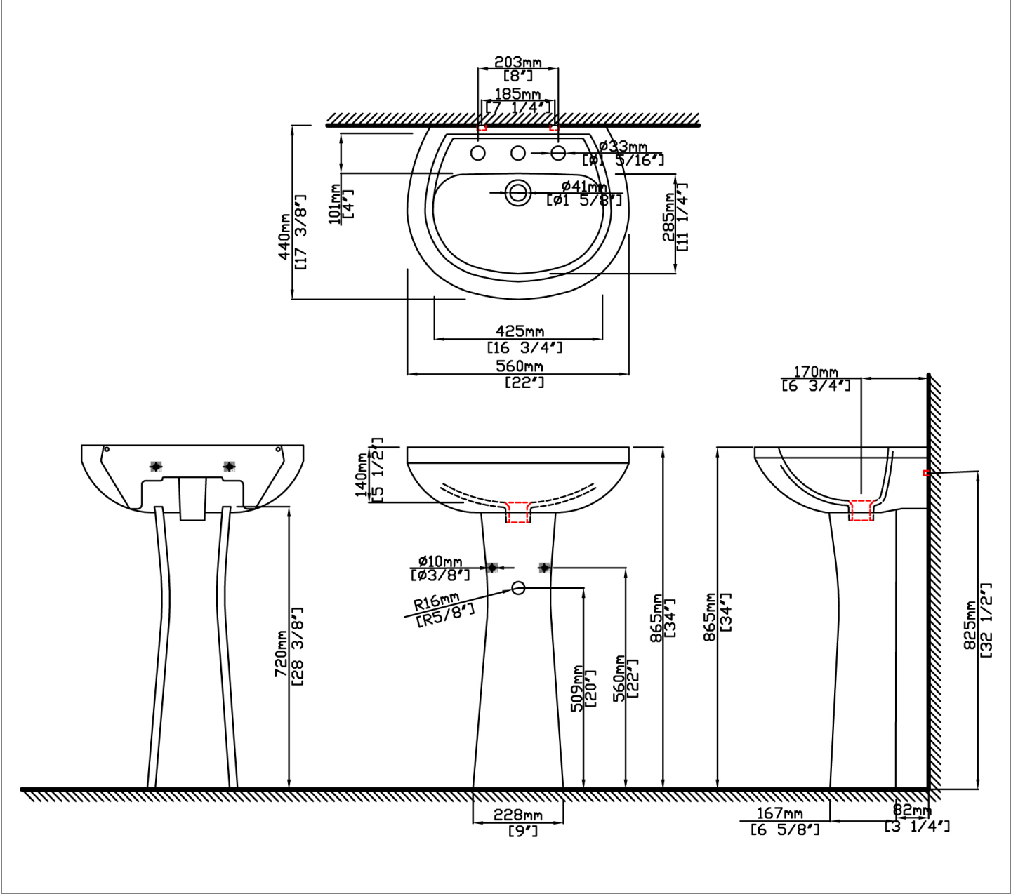
Dimensional Diagram
